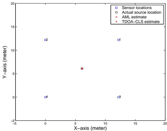
Figure 7. Source localization result of a music signal
