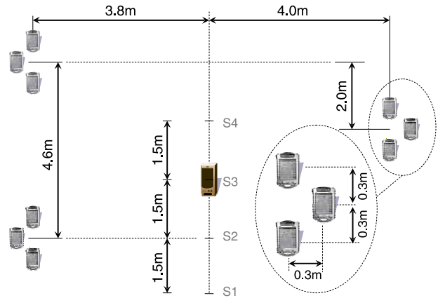
Figure 8. Array configuration 1
